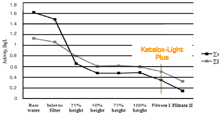
Changes in the radioactivity of water treated with Katalox-Light Plus
