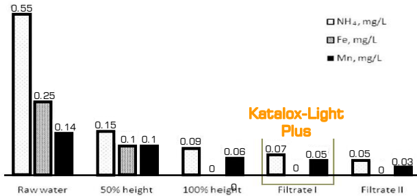
Changes in ammonia, total iron, and manganese content in the two-stage filtration system.
